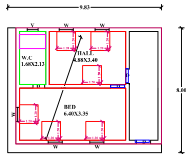
PROPOSED F.F.PLAN
