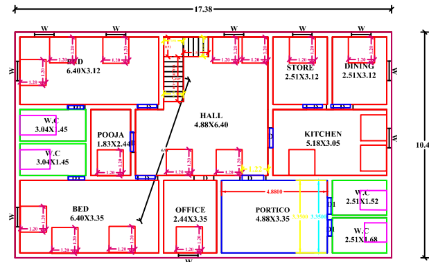
PROPOSED G.F.PLAN
