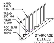
STAIRCASE DETAILS SCALE 1:50
