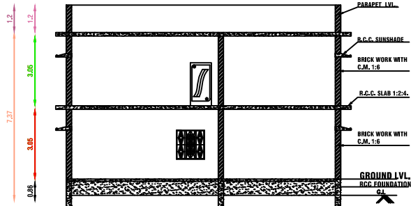
SECTION ON A-A & A'-A'
