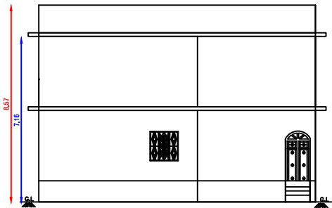
FRONT ELEVATION
