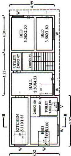
FIRST FLOOR PLAN (PROPOSED)
