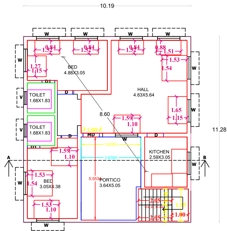
PLAN B
