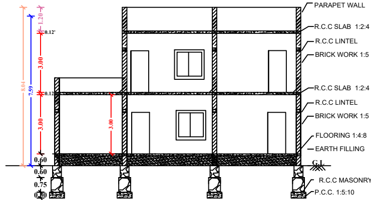
SECTION AB
