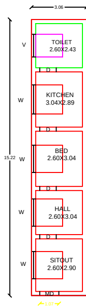
GROUND FLOOR PLAN
