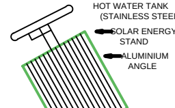
DETAILS OF SOLAR WATER HEATER
