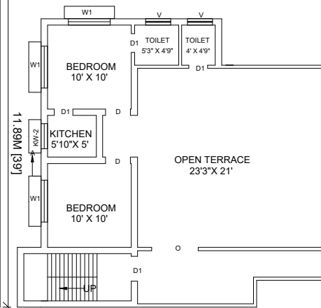
PRO.FIRST FLOOR
