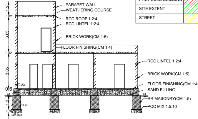
SECTION OF AB
