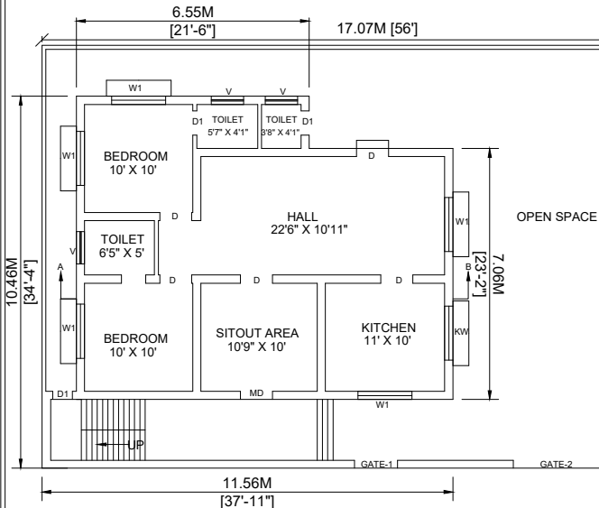
SITE CUM PRO.GROUND FLOOR
