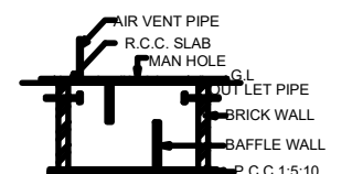
SECTION ON SEP.TANK
