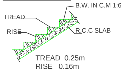
STAIR DETAILS
