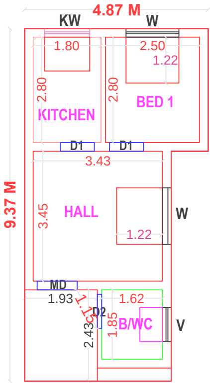
PLAN - GROUND FLOOR ( PROPOSED )
