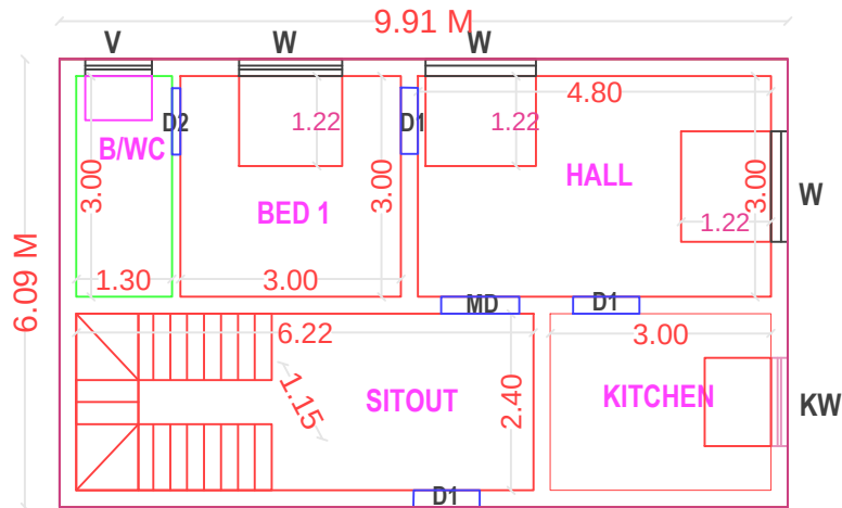
PLAN - GROUND FLOOR ( PROPOSED )
