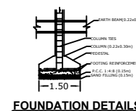
FOUNDATION DETAILS
