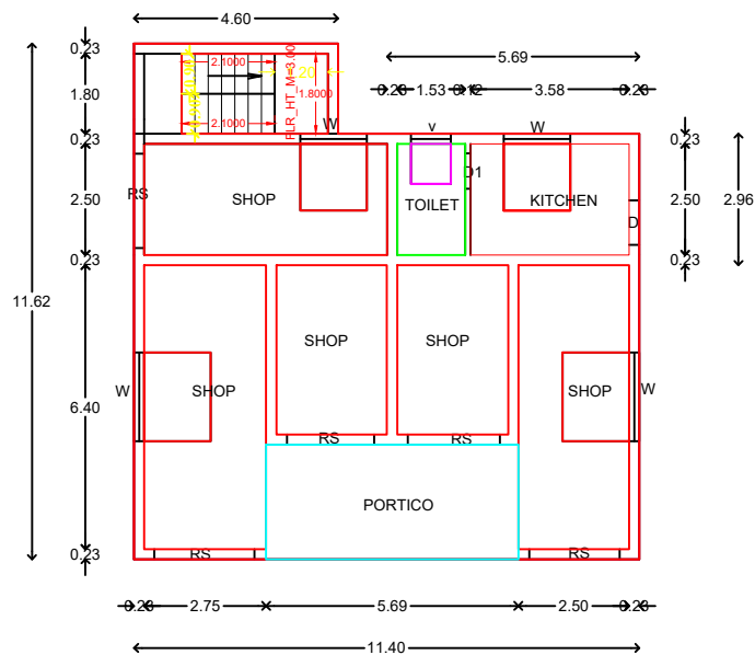
G.FLOOR PLAN
