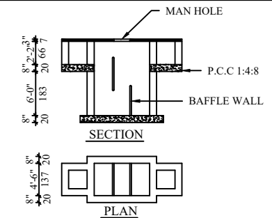
SEPTIC-TANK DETAIL
