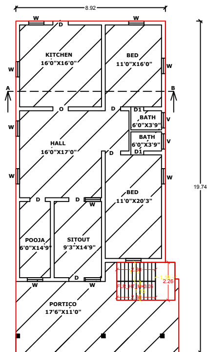
EXG.GROUND FLOOR PLAN
