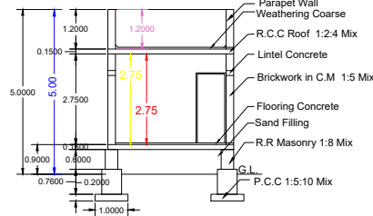
SECTION ON SS
