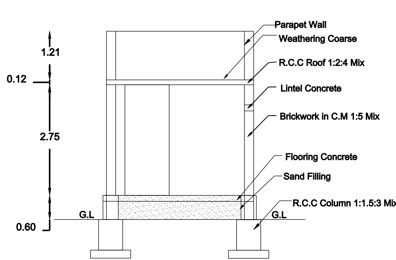
SECTION ON "SS"
