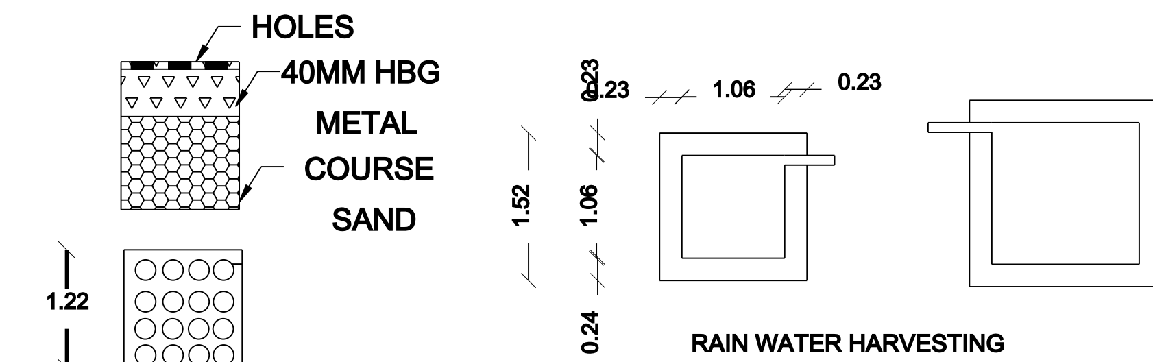
RAIN WATER COLLECTING TANK
