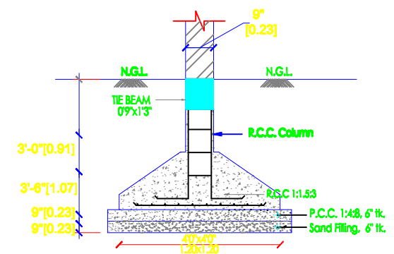
FOUNDATION DETAIL
