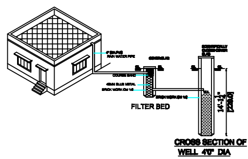
PRO.RAIN WATER SYSTEM
