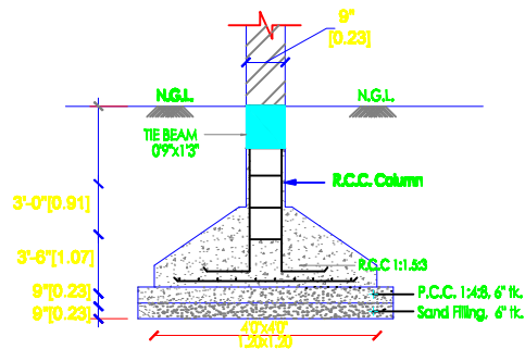
FOUNDATION DETAIL
