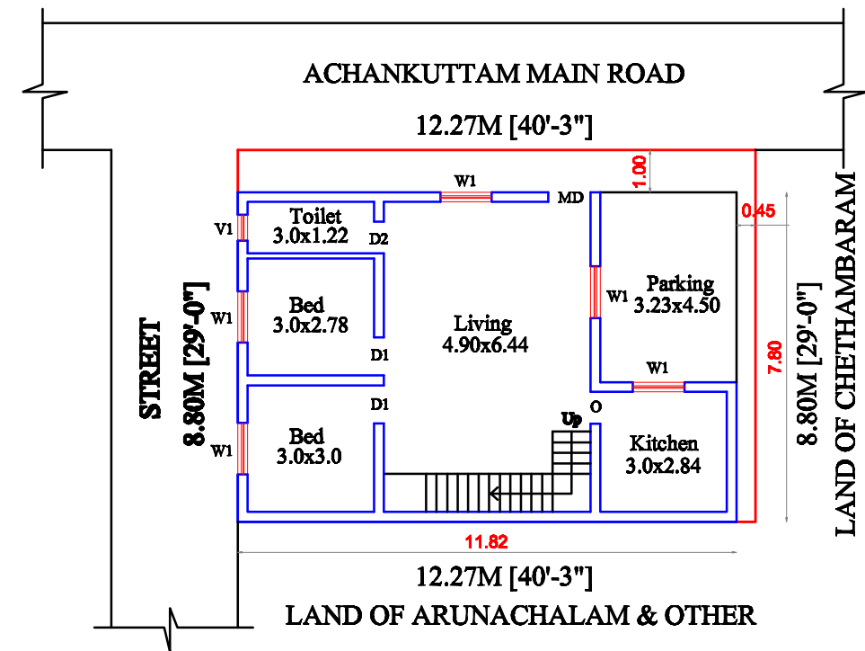
SITE CUM GROUND FLOOR PLAN
