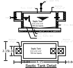
Septic Tank Detail
