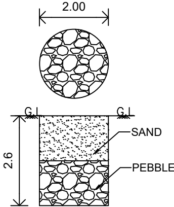
RAINWATER HARVESTING
