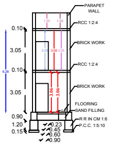
SECTION AB
