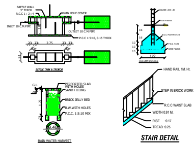
STAIR DETAIL
