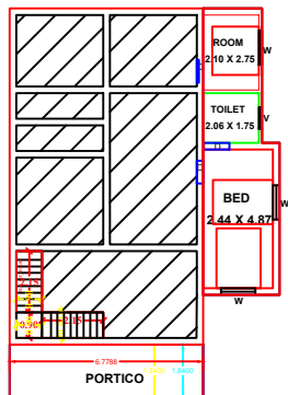
EXG & PRO GROUND FLOOR PLAN
