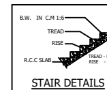
STAIR DETAILS
