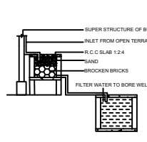
DETAILS OF FILTER BED & WELL
