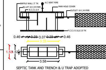
SEPTIC TANK AND TRENCH & U TRAP ADOPTED
