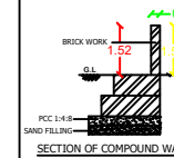
SECTION OF COMPOUND WALL
