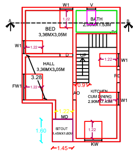
TYPICAL_FLOOR_PLAN=1
