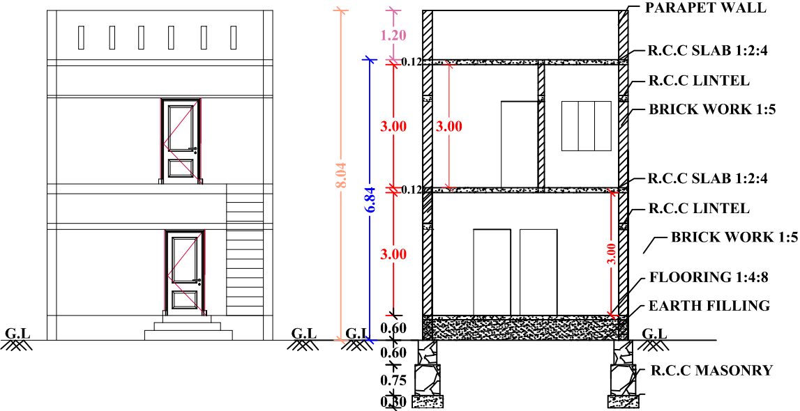
FRONT ELEVATION
