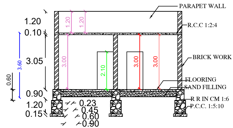
SECTION AB
