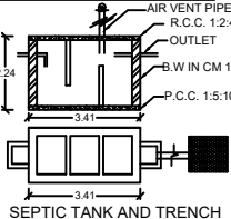
SEPTIC TANK AND TRENCH
