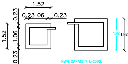
RAIN WATER COLLECTING TANK
