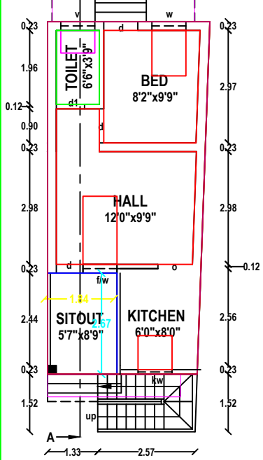
PLAN - GROUND FLOOR RESIDENCE
