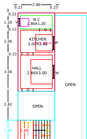
PRO FIRST FLOOR RESIDENTIAL PLAN
