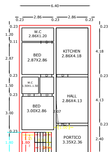
EXT GROUND FLOOR RESIDENTIAL PLAN
