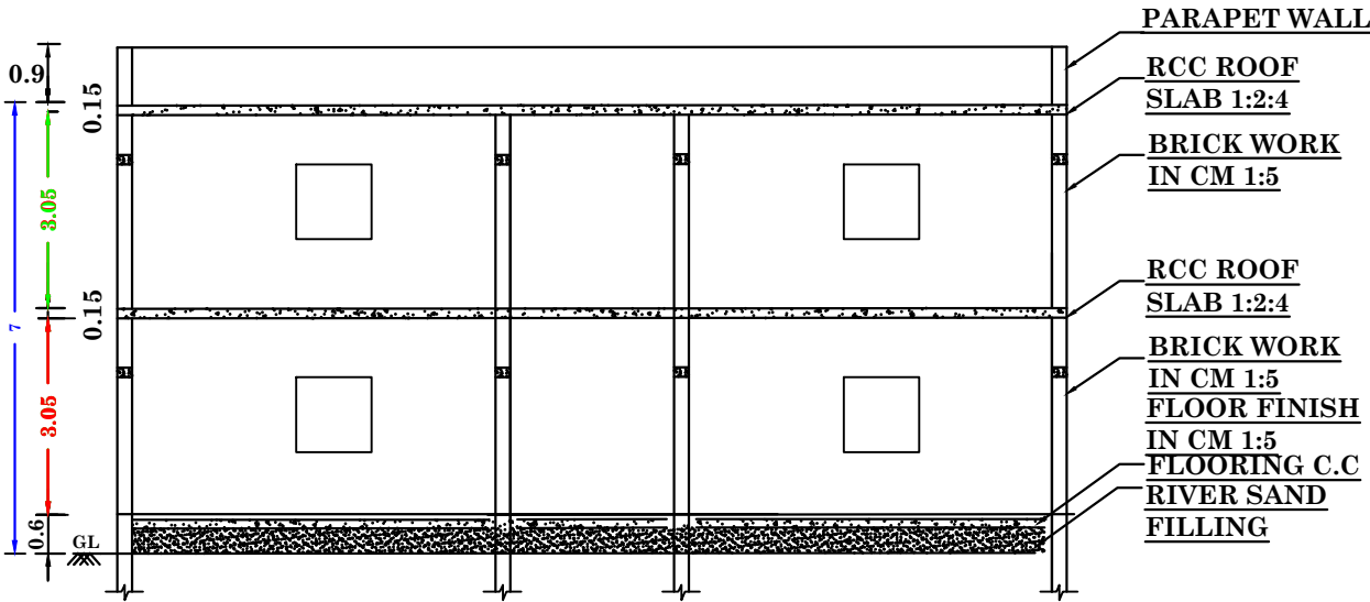
SECTION ON AA1
