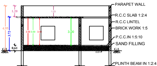
"SECTION 'AB'"
