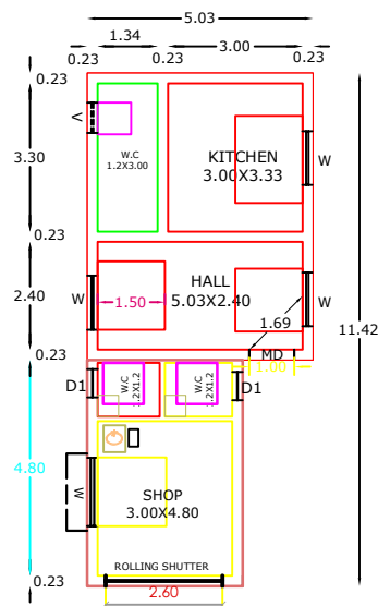
GROUND FLOOR COMMERCIAL CUM RESIDENTIAL PLAN
