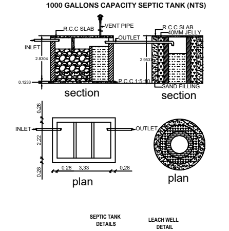
1000 GALLONS CAPACITY SEPTIC TANK (NTS)
