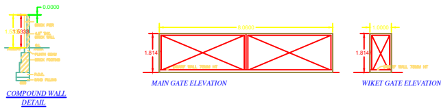
COMPOUND WALL DETAIL
