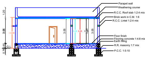
SECTION AB
