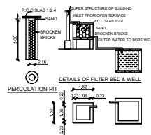
METAL COURSE SAND RAIN WATER COLLECTING TANK
