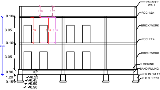
SECTION AB
