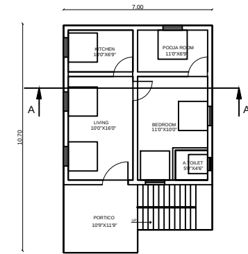
GF PLAN
