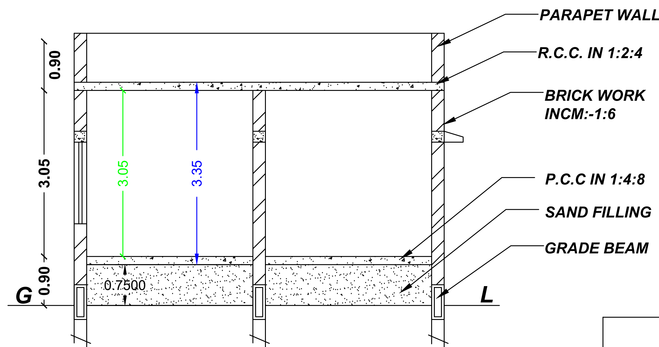
SECTION "AB"
