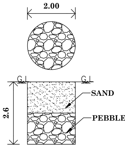
RAINWATER HARVESTING
