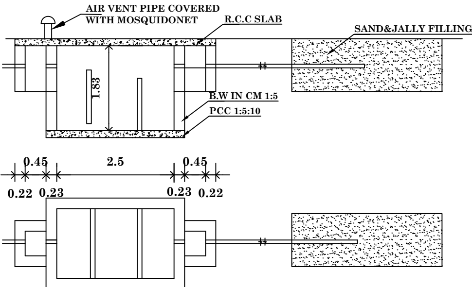
PLAN&SECTION OF SEPTIC TANK TRENCH
