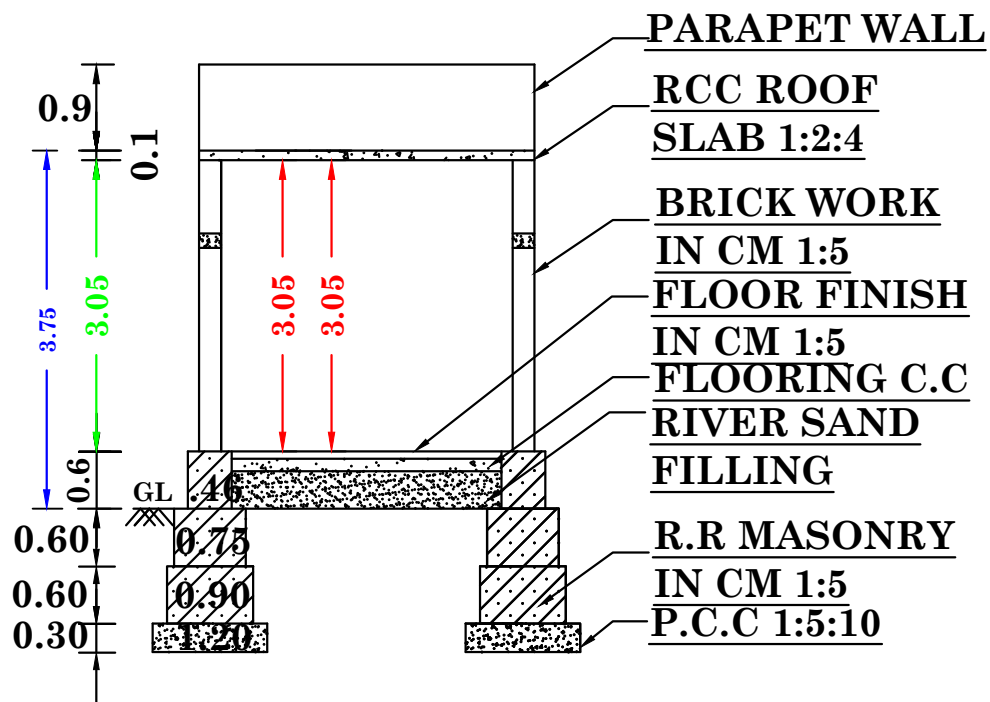
SECTION ON AA1
