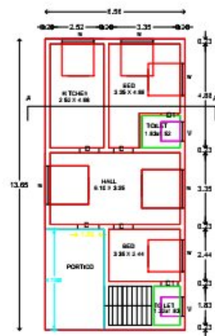
G.FLOOR PLAN
