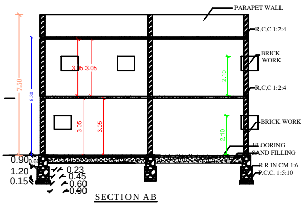
SECTION AB
