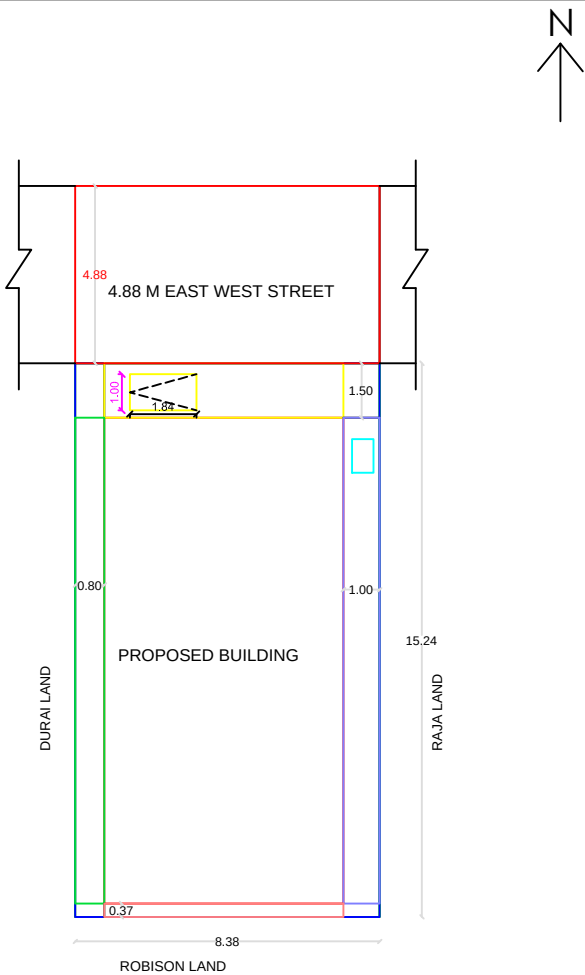
SITE PLAN
