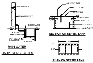
PLAN ON SEPTIC TANK
