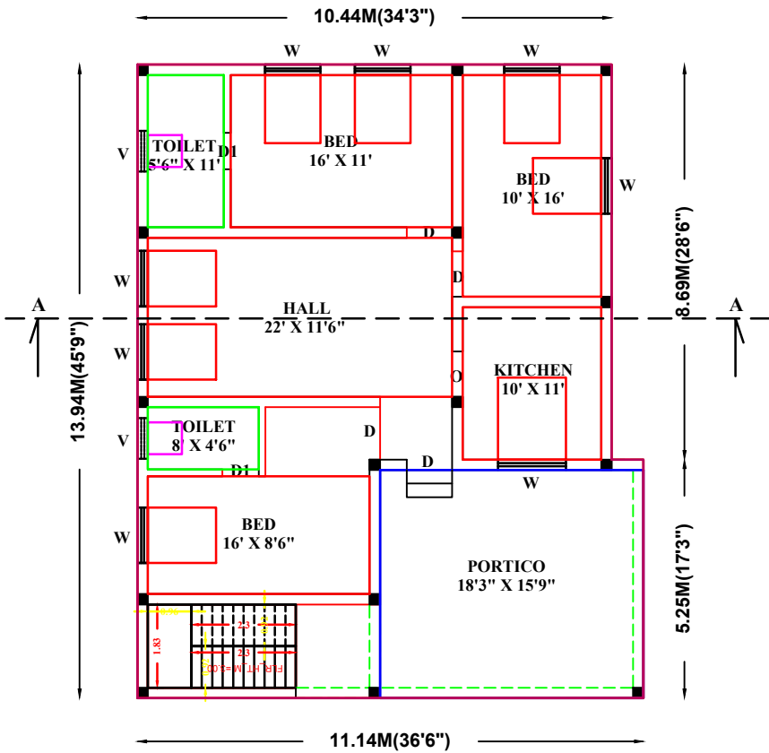
PLAN
