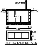
SEPTIC TANK DETAILS
