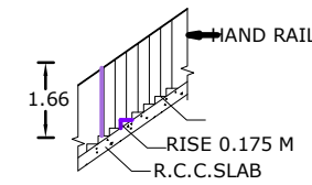
STAIRCASE
