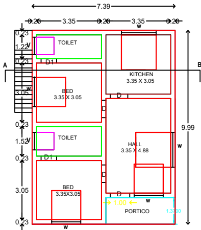
G.FLOOR PLAN
