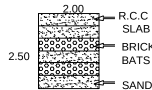
SECTION ON C - D
