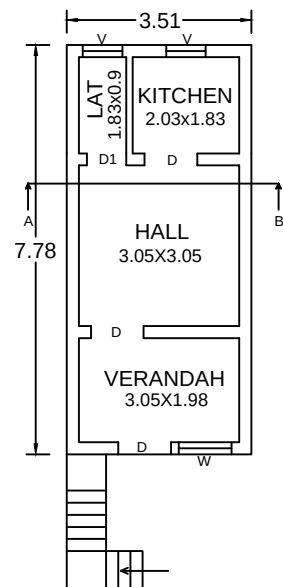
FLOOR PLAN
