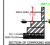
SECTION OF COMPOUND WALL
