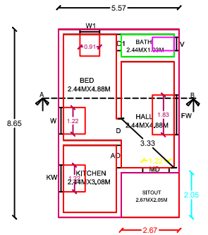
TYPICAL_FLOOR_PLAN=1
