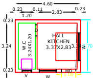
GROUND FLOOR PLAN
