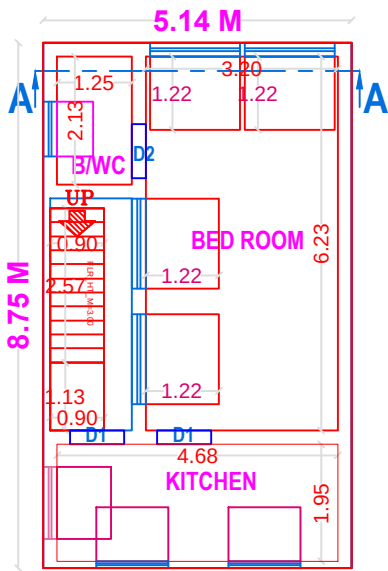
PLAN - FIRST FLOOR ( PROPOSED )
