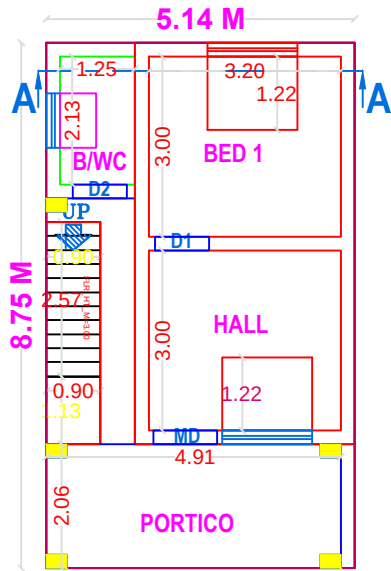
PLAN - GROUND FLOOR ( ADD. PROPOSED )
